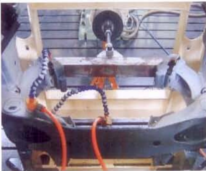
Engine Mount 耐久试验
